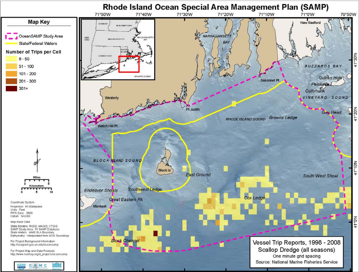
Figure 5.21. Scallop dredging areas based on NMFS Vessel Trip Reports, 1998 - 2008.
