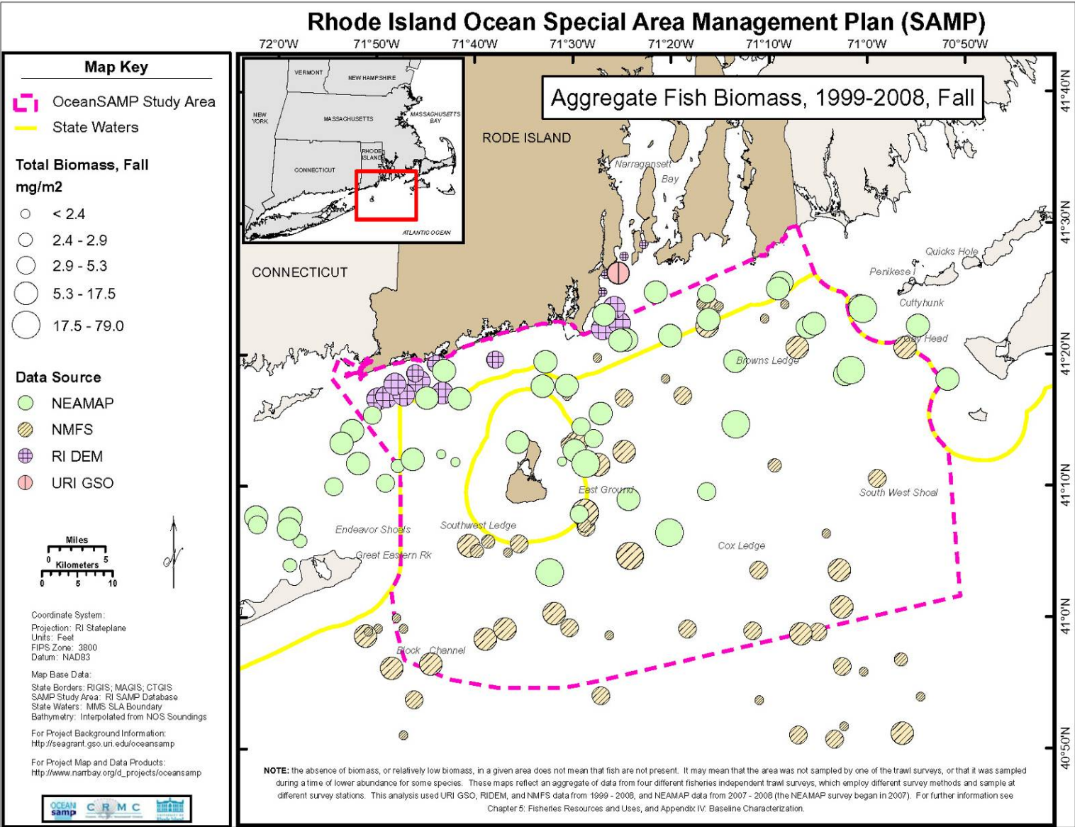
Figure 5.4. Aggregate fish biomass, 1999-2008, fall.
